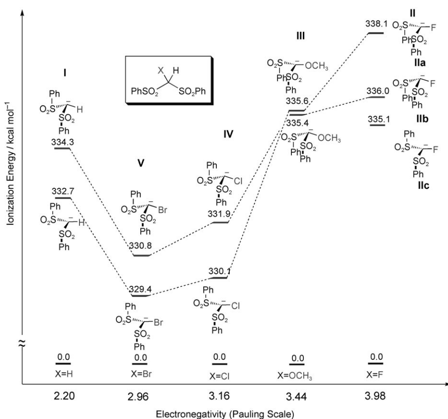
Figure 3. Gas-phase proton affinities (ionization energy/electronegativity profile) of carbanions I-V .
