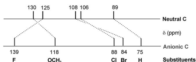
Figure 4. Calculated 13 C NMR chemical shifts of the \alpha -C (carbanionic carbon) in I–V and the corresponding neutral molecules.
